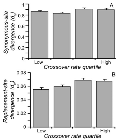
Figure 3. Lineage-specific synonymous-site (A) and replacement-site divergence (B) for quartiles of recombination rate in C. briggsae , in genome comparisons with C. remanei and C. elegans as outgroups. ANOVA models that include recombination rate, codon bias, background nucleotide composition, chromosome of origin, divergence, and their first-order interactions provide statistical support for the positive d_s -recombination and d_N -recombination associations. Error bars indicate \pm 1 standard error.
