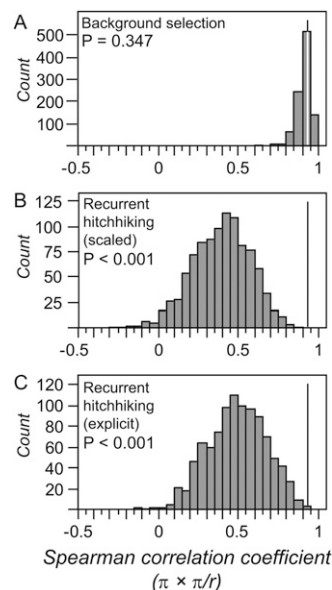
Figure 7. Distribution of correlation coefficients between neutral polymorphism and the polymorphism-recombination rate ratio ( R_{p-r} ). The observed correlation (Spearman rank correlation = 0.930; vertical line) falls within the distribution simulated for background selection (A), but not for the genetic hitchhiking model (B,C). The hitchhiking model in B uses scaled output of neutral coalescent simulations, whereas C uses direct simulation of a recurrent sweep process (Jensen et al. 2008). Simulations for A assume \pi_0 = 0.0138 and for B assume \pi_0 = 0.0486 (similar distributions result when \pi_0 are identical), as well as c = 0.000158 , a = 7.67 \times 10^{-9} , 800-bp loci, \mu = 1.7 \times 10^{-9} (see Supplemental Fig. 2), and the observed fine-scale crossover rates for 22 loci. Parameters from both A and B are based on least-squares fitting of analytical selection models. Explicit recurrent hitchhiking simulations for C are based on \pi_0 = 0.035 , c = 0.000158 , s = 0.001 , \lambda = 1 \times 10^{-6} , and fine-scale crossover rates for 22 loci.
